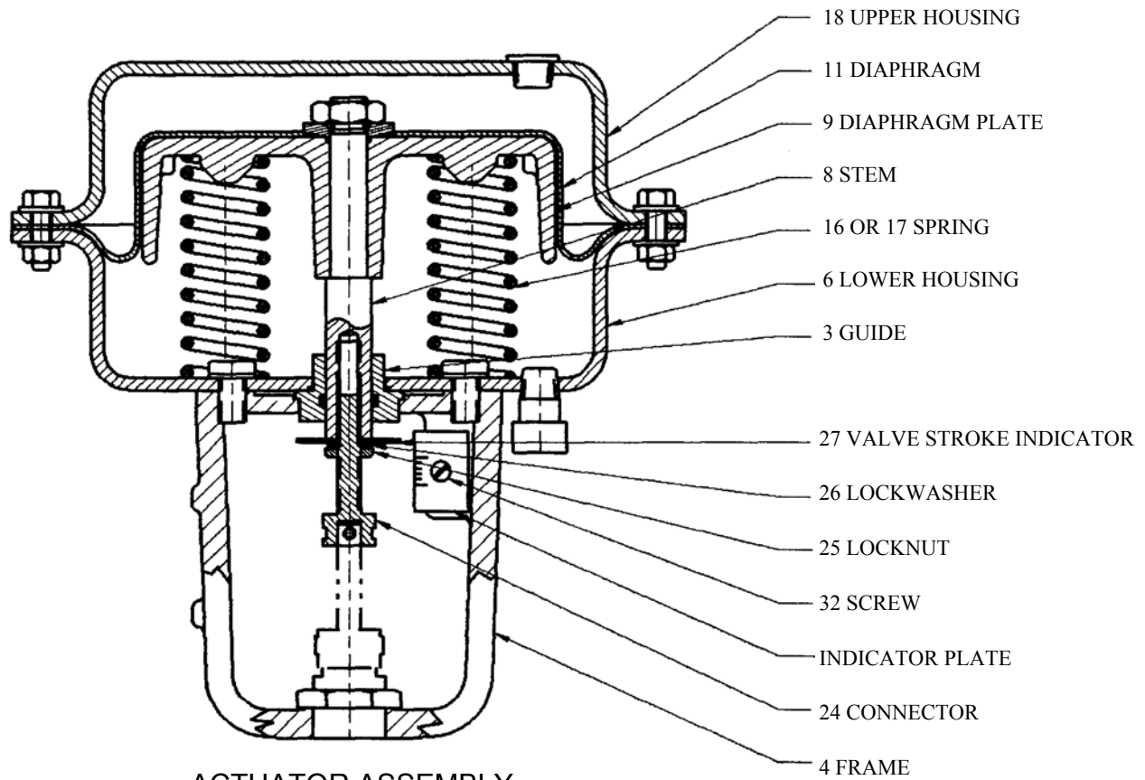
ACTUATOR ASSEMBLY VC-230A (DIRECT-ACTING)
